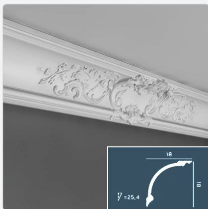
Orac Luxxus C338A
