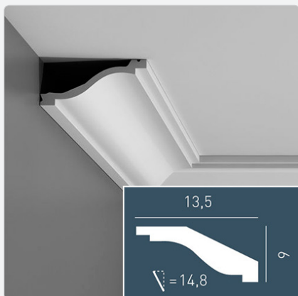
Orac Luxxus C331
